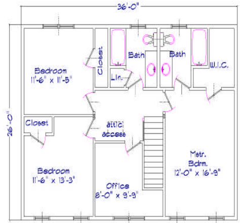
Second Floor Plan Approximate living Area: 936 s.f.
