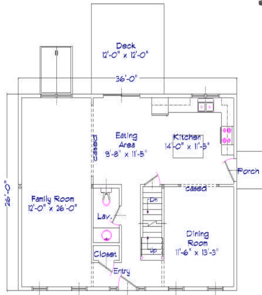
First Floor Plan Approximate living Area: 936 s.f.
