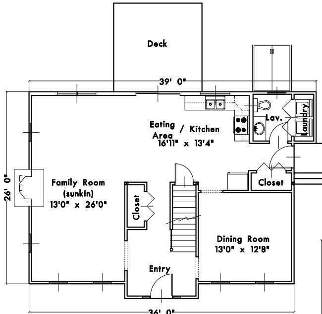
FIRST FLOOR PLAN Approximate Living Area: 956 s.f.
