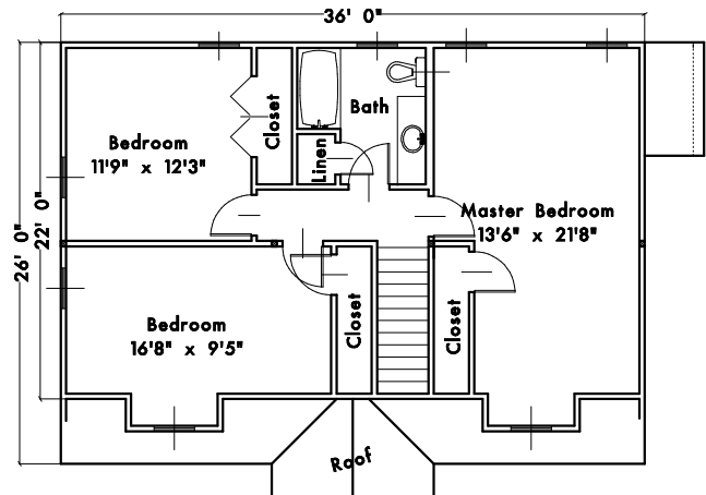
SECOND FLOOR PLAN Approximate Living Area: 816 s.f.
