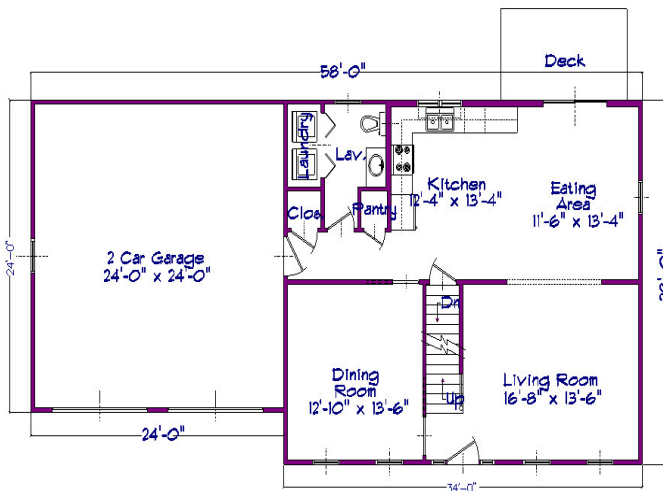
First Floor Plan Approximate Living Area: 952 s.f.
