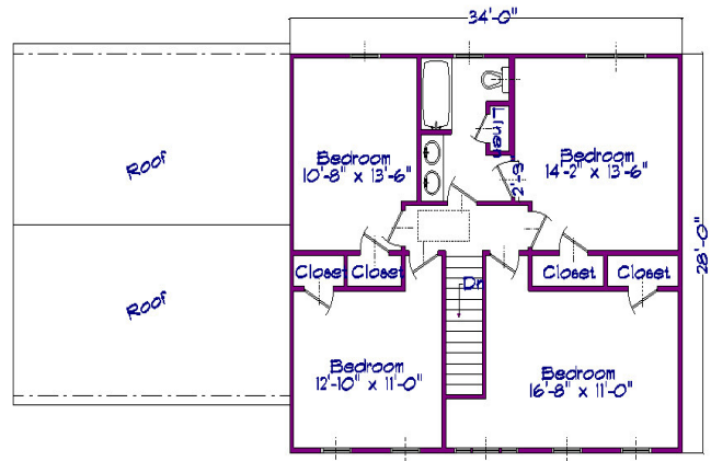
Second Floor Plan Approximate Living Area: 952 s.f.
