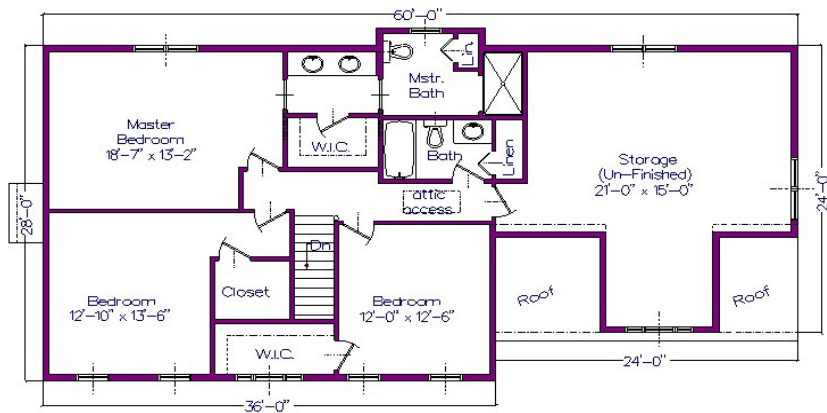
Second Floor Plan Approximate Living Area: 1,498 s.f.
