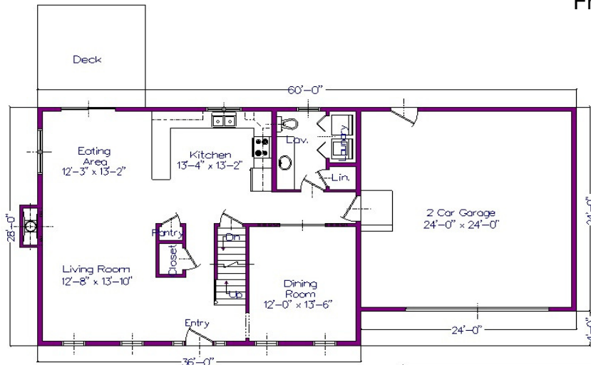
1st Floor Plan Approximate Living Area: 1,008 s.f.
